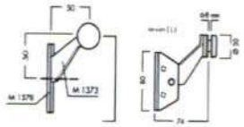
HB-328 玻璃爪 (单爪) Glass/panel vetainer
