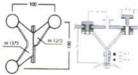
HB-330 玻璃爪 (三爪) Glass/panel vetainer
