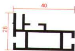
HB-347 40单面弹力布边框 Single-sided frame Lenght:6m
