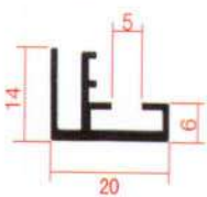
HB-346 20画框 Frame extrusion/20 Lenght:6m
