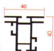
HB-348 40双面弹力布边框 Single-sided frame Lenght:6m
