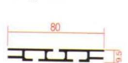
HB-350 80双面弹力布边框 Double-sided frame Lenght:6m
