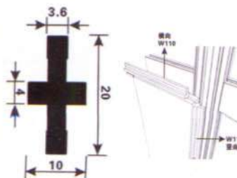
HB-338 十字铝 Separate from panels Length: 6m
