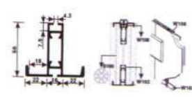
HB-334 双面墙型材 Beam Extrusion Length: 6m
