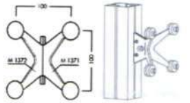
HB-331 玻璃爪 (四爪) Glass/panel vetainer
