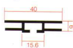
HB-349 40弹力布边框 Frame extrusion Lenght:6m
