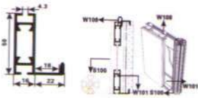
HB-333 单面墙型材 Beam Extrusion Length: 6m
